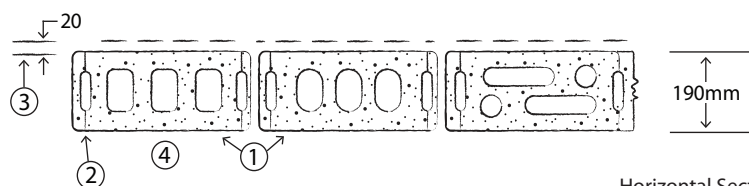
Horizontal Section Bearing or Non-bearing Wall
