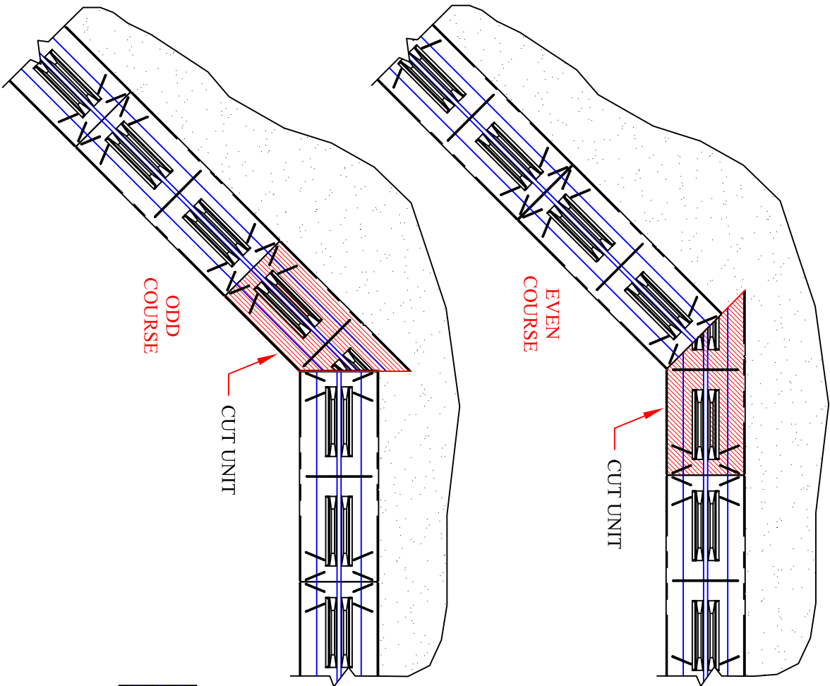
PROTERRA STANDARD UNIT
