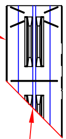
CUTBACK AT 45 DEGREE ANGLE FROM THE FRONT FACE
