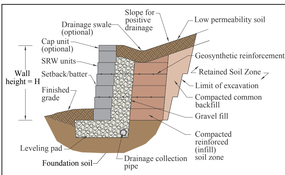
Figure 1—Reinforced Segmental Retaining Wall System Components
